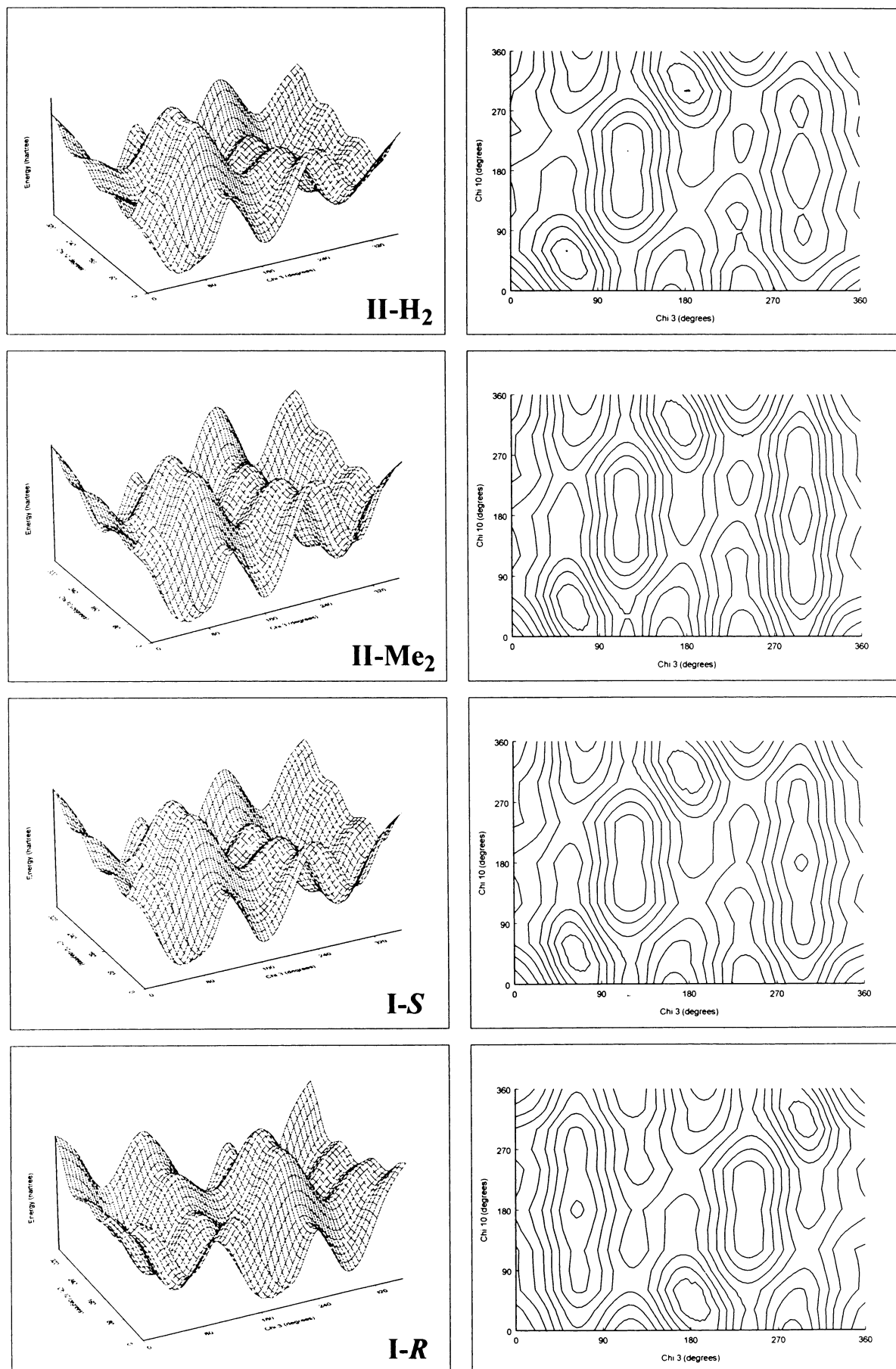
Figure 13. PES [ E = f(\chi_3, \chi_{10}) ] for carbazole-containing analogues (from top to bottom): (2-hydroxyethoxy)carbazol ( II-H 2 ), (2-hydroxy-2-methylethoxy)carbazol ( II-Me 2 ), S -4-(2-hydroxypropoxy)carbazol ( I-S ), and R -4-(2-hydroxypropoxy)carbazol ( I-R ). The torsional angles \chi_1 and \chi_2 were frozen at 180.00^\circ during the cross-sectional calculations of the PEHS.
